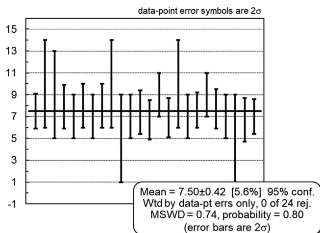
Fig. 9. Weight means U-Pb age of the sample #13Ge-04 from the Mtkvari pyroclastic flow.
