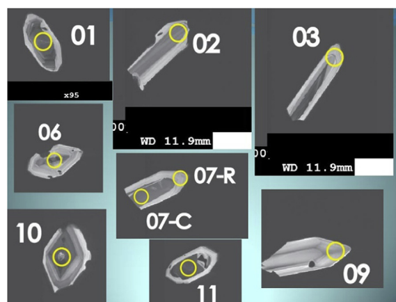
Fig. 7. Part of CL images of the zircon grains of the Mtkvari ignimbrites flow. Sample #13Ge-04.
