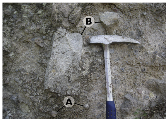
Fig. 5. Exposure of the Mtkvari pyroclastic flow on the right side of the Vardzia rock-cut city. Lithoclasts characterizing the horizon (0.2–3.5 cm). B- Rare rutaceous lithoclasts.
