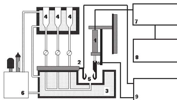
Fig. 1. Block diagram of the mechanotron unit: 1-mechanotron, 2-mechanism of tension and calibration; 3-thermostated chamber; 4-flasks for feeding the substances under study; 5-working chamber; 6-ultrathermostat; 7-amplifier; 8-recorder; 9-electrostimulator
